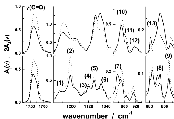
Fig. 2. Selected regions of the polarized IR spectra, A_{\parallel}(v) (solid lines) and 2A_{\perp}(v) (dotted line), of POPC in the absence (above) and presence of \text{Zn}^{2+} (below, R_{Z/L} \approx 1 ) in a \text{D}_2\text{O} atmosphere of \text{RH} = 71\% at T = 30^\circ\text{C} . The numbers are assigned to the absorption bands of the phosphate (below) and trimethylammonium (above) groups (cf. Table 1).
