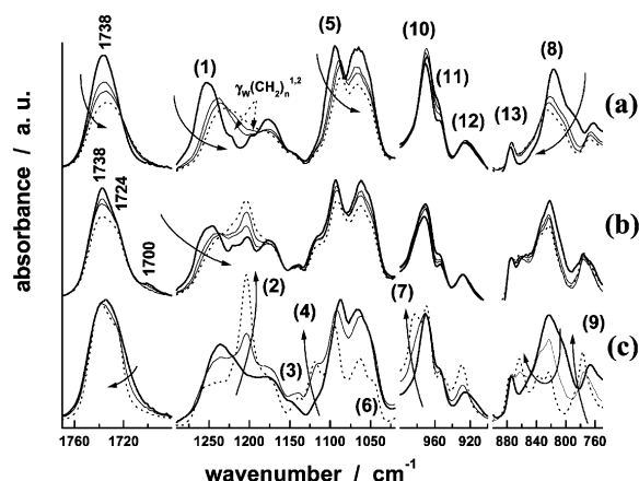
Fig. 1. Selected regions of the IR spectrum of POPC in the absence (a) and presence of \text{Zn}^{2+} (b, R_{\text{Z/L}} = 0.7 ) at variable \text{RH}(\text{D}_2\text{O}) = 5, 50, 71 and 89\% , and at a variable molar ratio of \text{ZnCl}_2 -to-POPC, R_{\text{Z/L}} = 0, 0.7 and 1 (c, \text{RH} = 71\% ). The temperature was T = 30^\circ\text{C} . The arrows indicate spectral shifts which are induced either by progressive hydration (a and b) or by the binding of \text{Zn}^{2+} (c). The numbers correspond to the vibrational modes which are assigned in Table 1.
