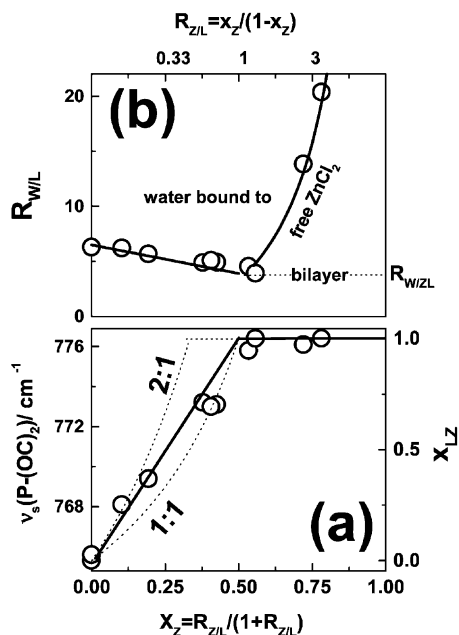
Fig. 3. Center of gravity of the \nu_{\text{s}}(\text{P}(\text{OC})_2) band of POPC (part a) and the number of water molecules per lipid, R_{\text{w/L}} (part b, see below), as a function of the mole fraction of \text{ZnCl}_2 , x_{\text{z}} , at \text{RH} = 71\% . R_{\text{w/L}} has been estimated from the integrated intensity of the \nu_{13}(\text{OD}) band of water (see below). The right axis in part (a) gives the mole fraction of the lipid–zinc complex x_{\text{LZ}} . The dotted lines in part (a) refer to a 2:1 (lipid: \text{Zn}^{2+} ) and 1:1 stoichiometry of the complex [see Appendix A, Eq. (A5)]. The solid lines refer to the model of strong binding (cf. Appendices A and B).
